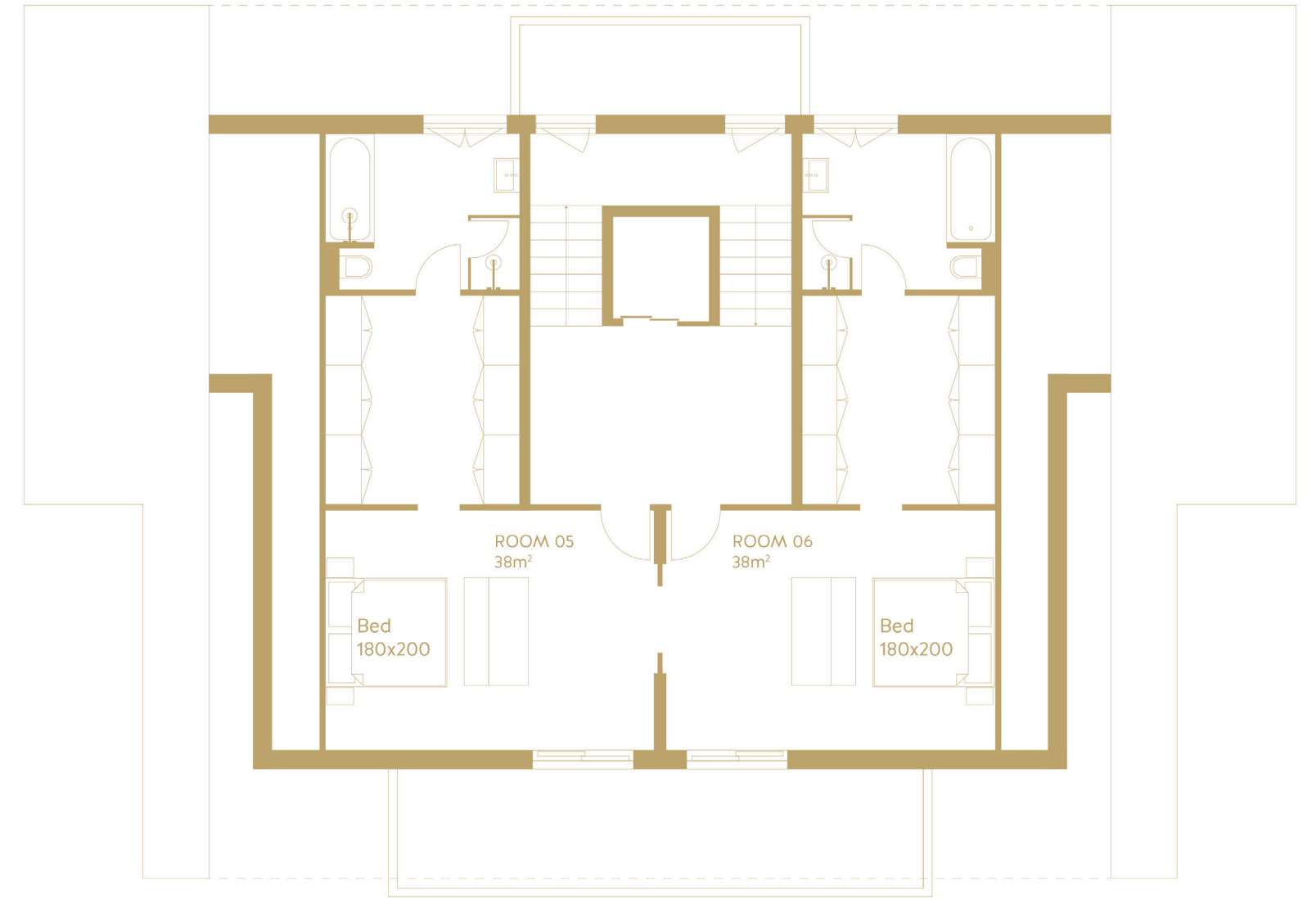
CRANS-MONTANA - CHALET TWO - 2 ND FLOOR
